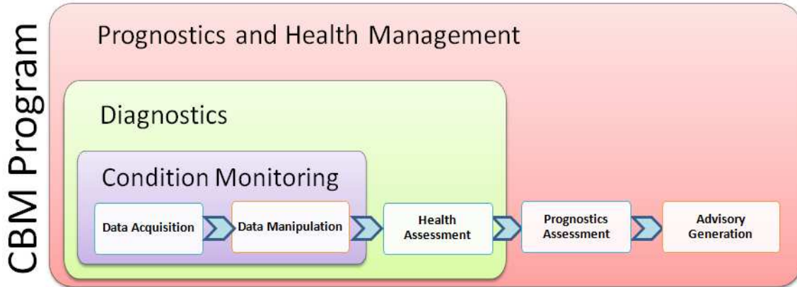
Figure 1.2 Functional layers of CBM
